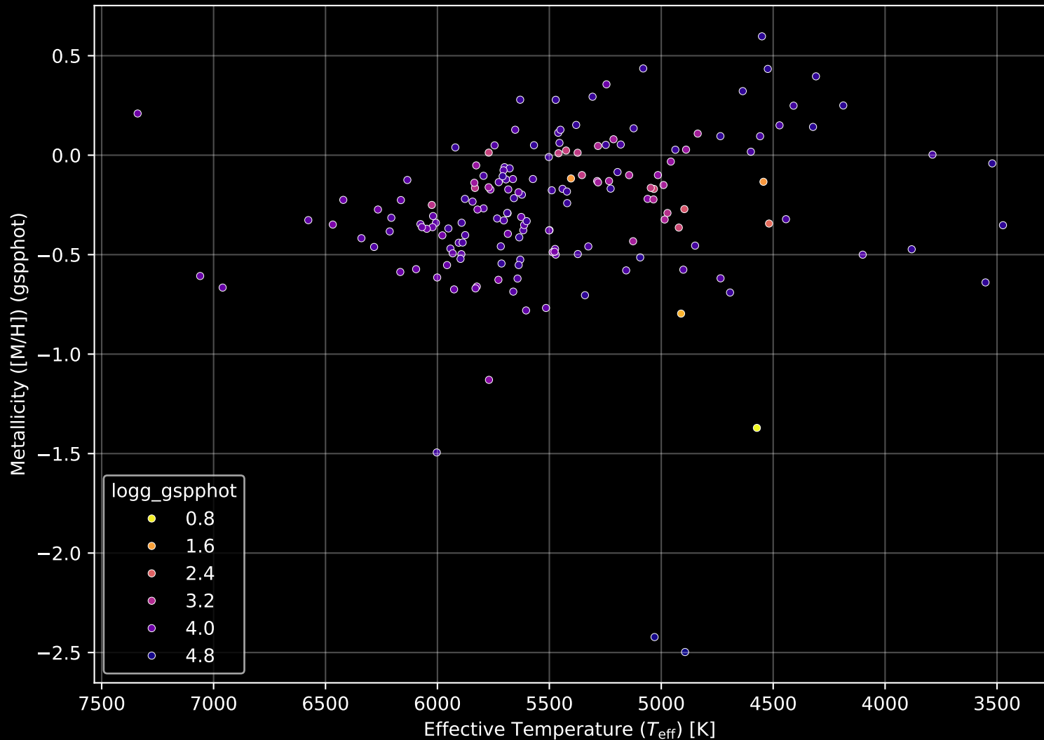
APOGEE DR17 Field: [053+58_MGA] Stellar Population Parameters (n= 169)
