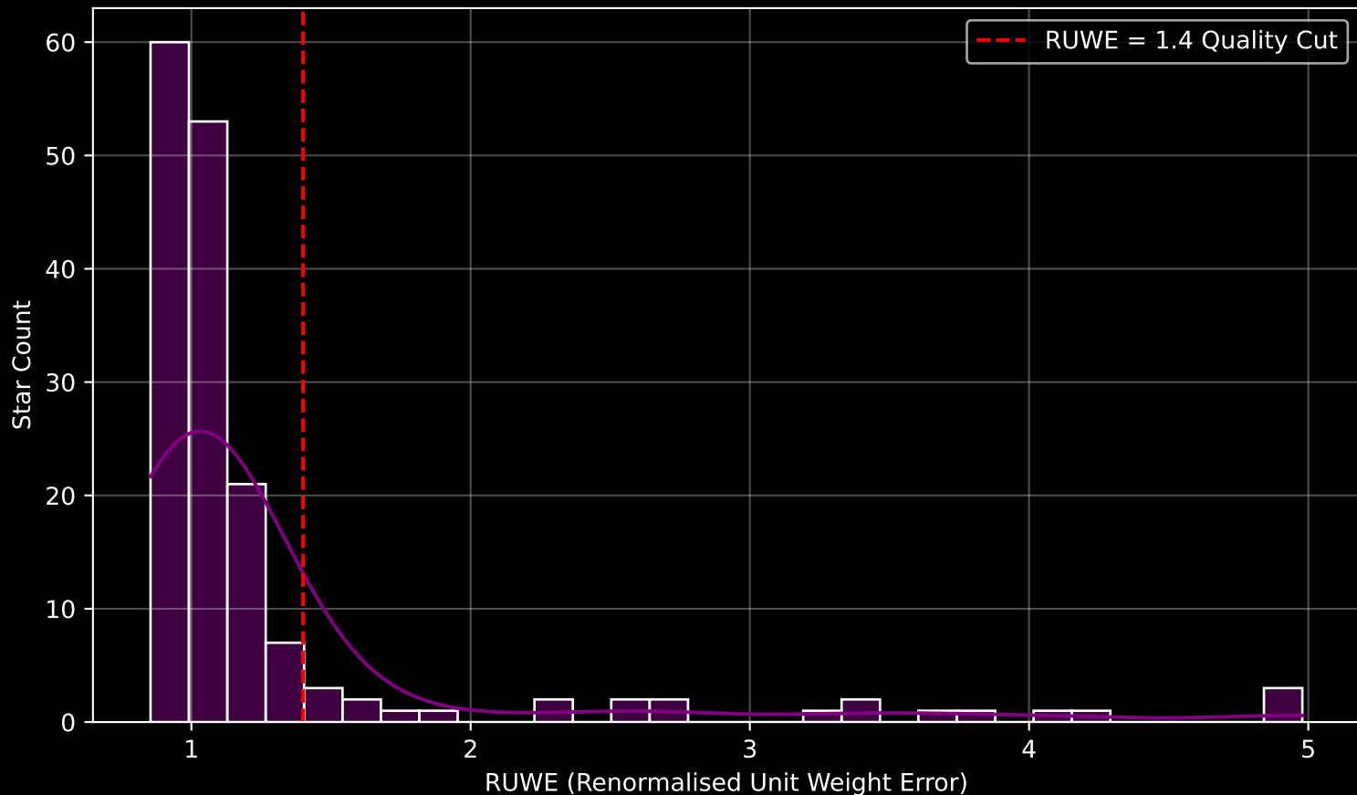
GAPOGEE DR17 Field [053+58_MGA] RUWE Distribution (n= 164)
