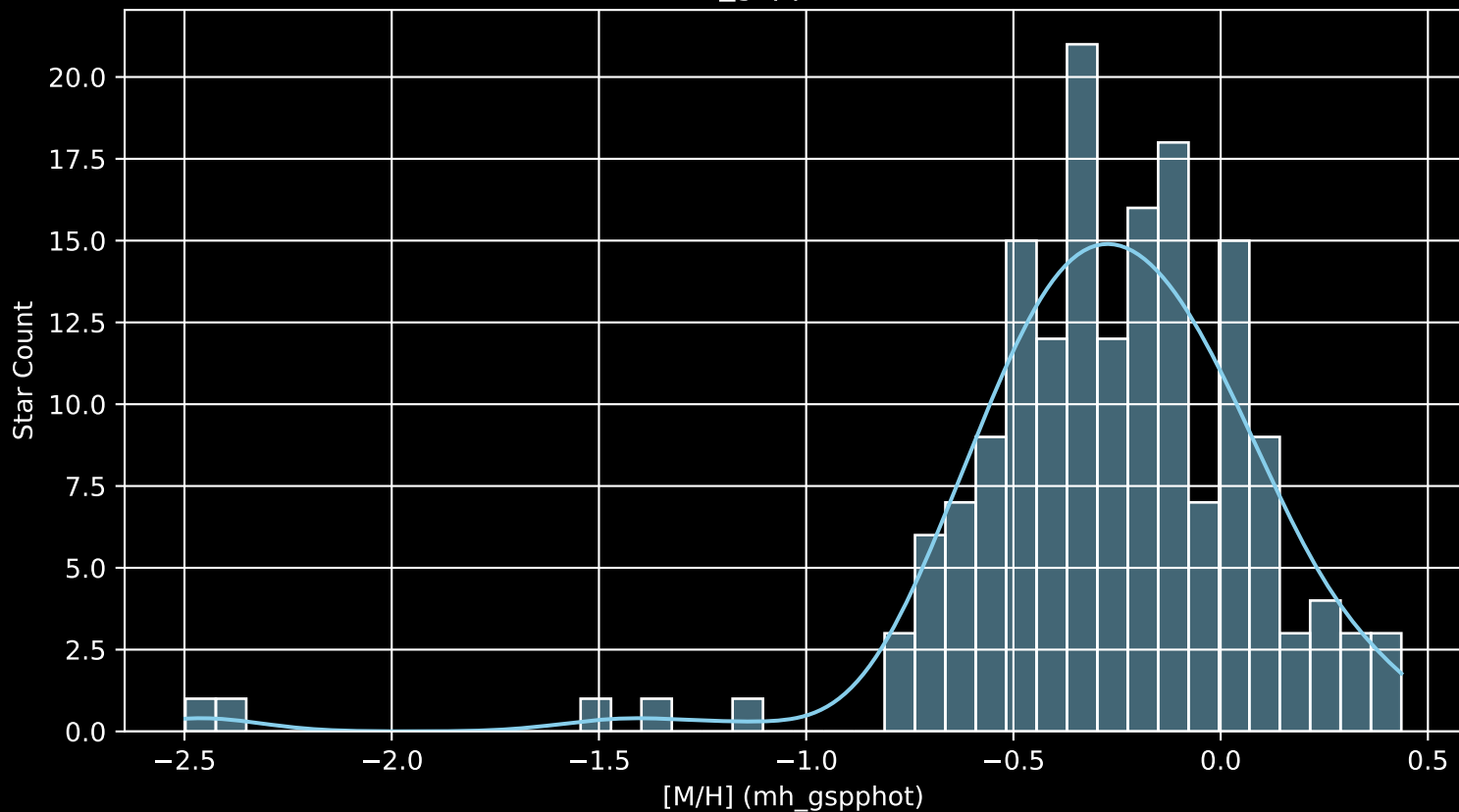
APOGEE DR17 Field: [053+58_MGA [M/H] (mh_gspphot) (n= 168)
