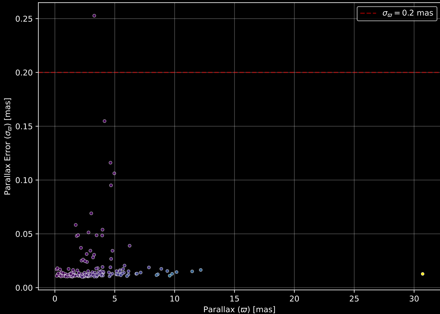
APOGEE DR17 Field: [053+58_MGA] Parallax Quality (n= 169)
