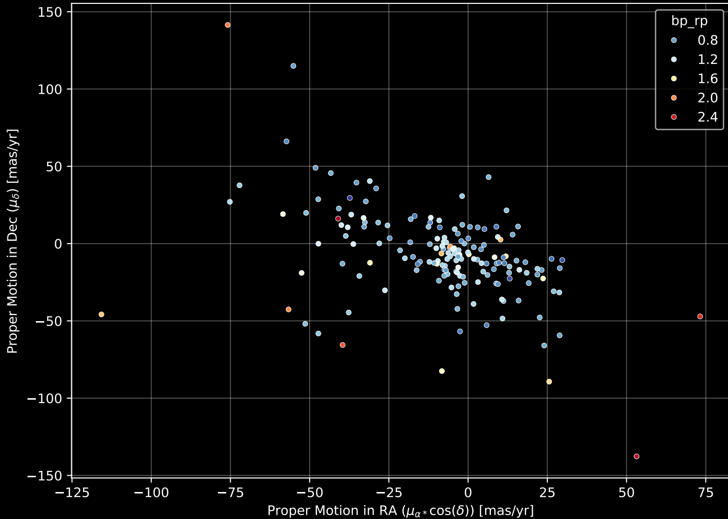
APOGEE DR17 Field: [053+58_MGA] Proper Motion Diagram (n= 169)
