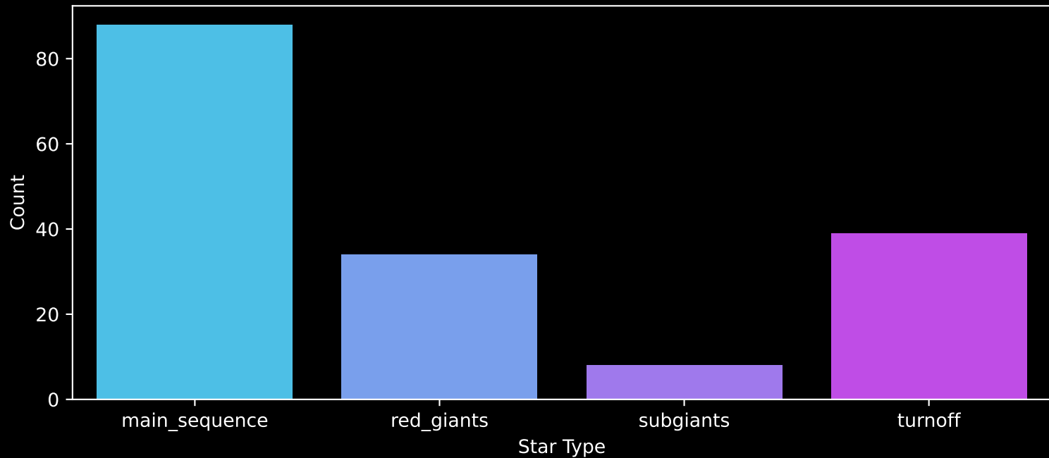
APOGEE DR17 Field: [053+58_MGA] Count plot of Star Type
